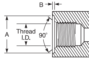
Female Types A & B
