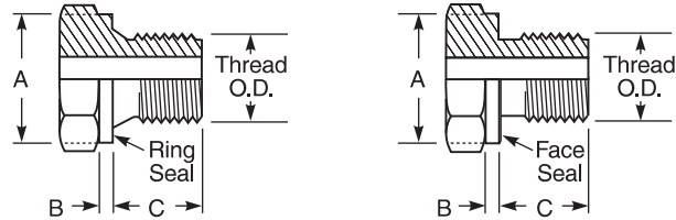
Male Type A
